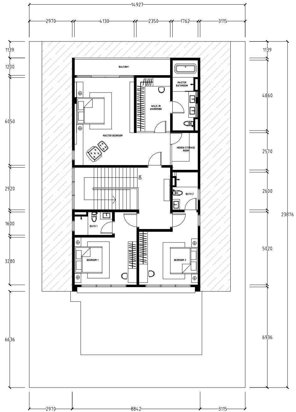
FURNITURE LAYOUT PLAN 1ST FLOOR
