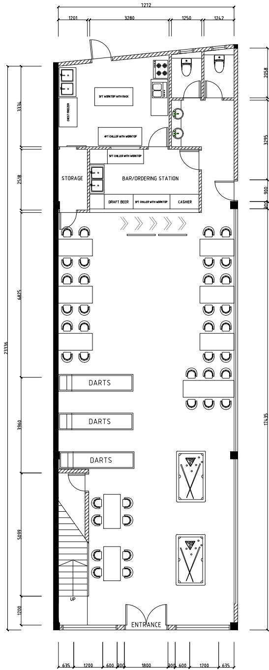
GF FURNITURE LAYOUT PLAN
